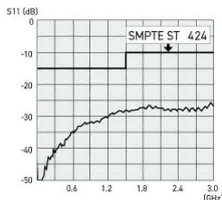
Patch Through (Return Loss for MCVJ-W)
