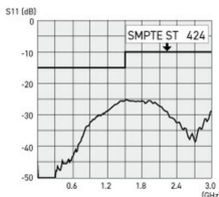
Normal Through (Return Loss for MCVJ-W)
