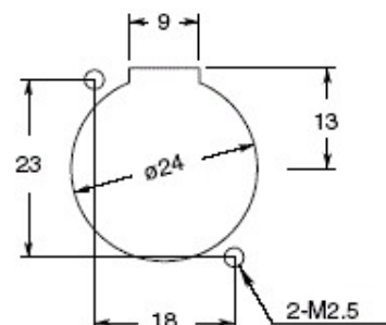
Flush-Mount Hole
