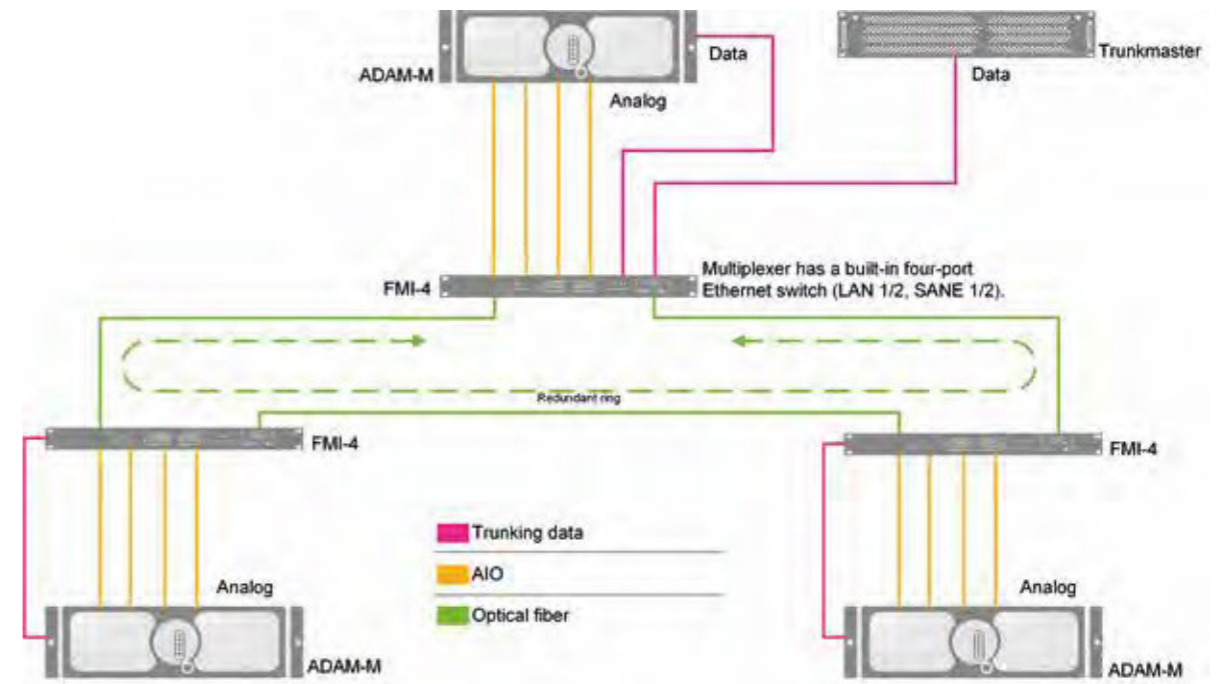
Figure 1. Non-redundant trunking application using analog connections (AIO). FMI-4 multiplexers are used to create a redundant transmission backbone.
