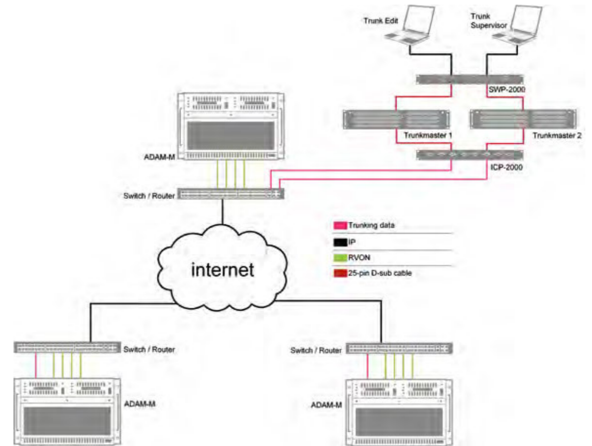
Figure 2. Redundant trunking application using audio over IP (RTS Voice Over Network, RVON). One of the Trunkmasters is a backup to the other.
