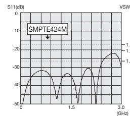
Return loss for BCP-C6HD
