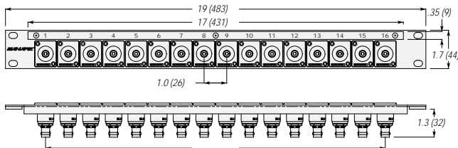
161U-RJRU 16ea 75Ω Type RCA-BNC Jacks Insulator Colors: Red, Green, Blue, Yellow, White
