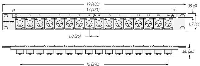
161U-X2F 16ea XLR3 Male-Solder Jacks
