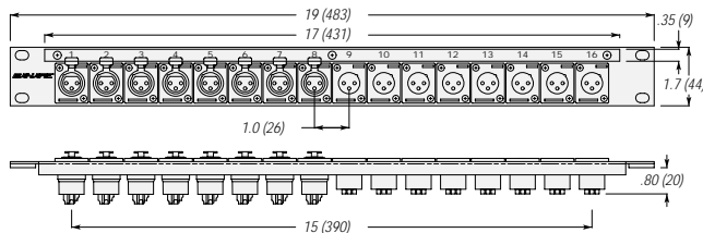
161U-X12F 8ea XLR3 Male & Female-Solder Jacks
